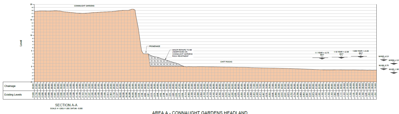
Figure 13: Frontage A preferred option
