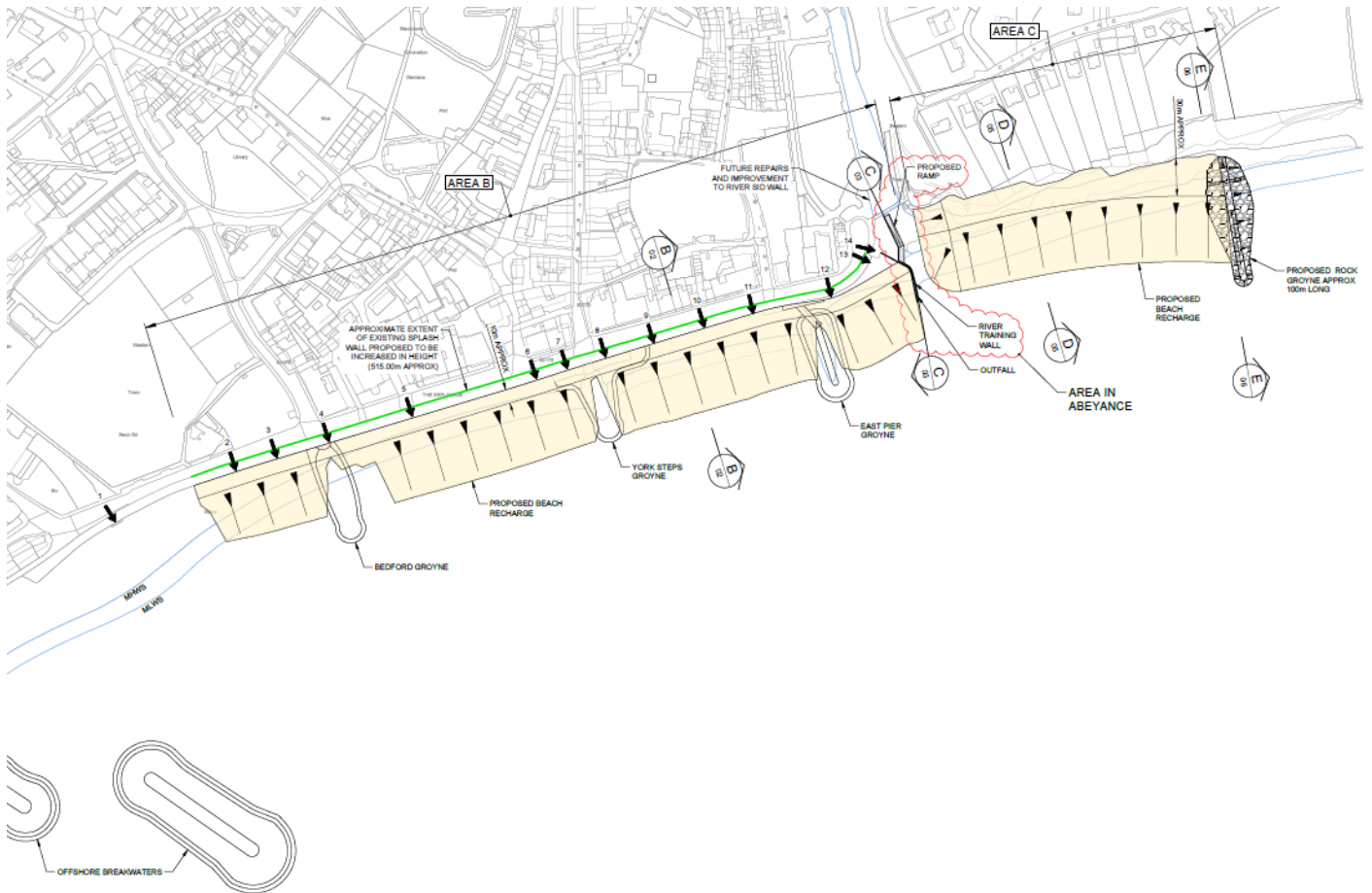
Figure 15: Existing and Proposed Splash Wall.
