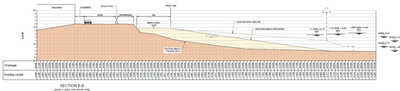
Figure 14: Sidmouth Town design beach.
