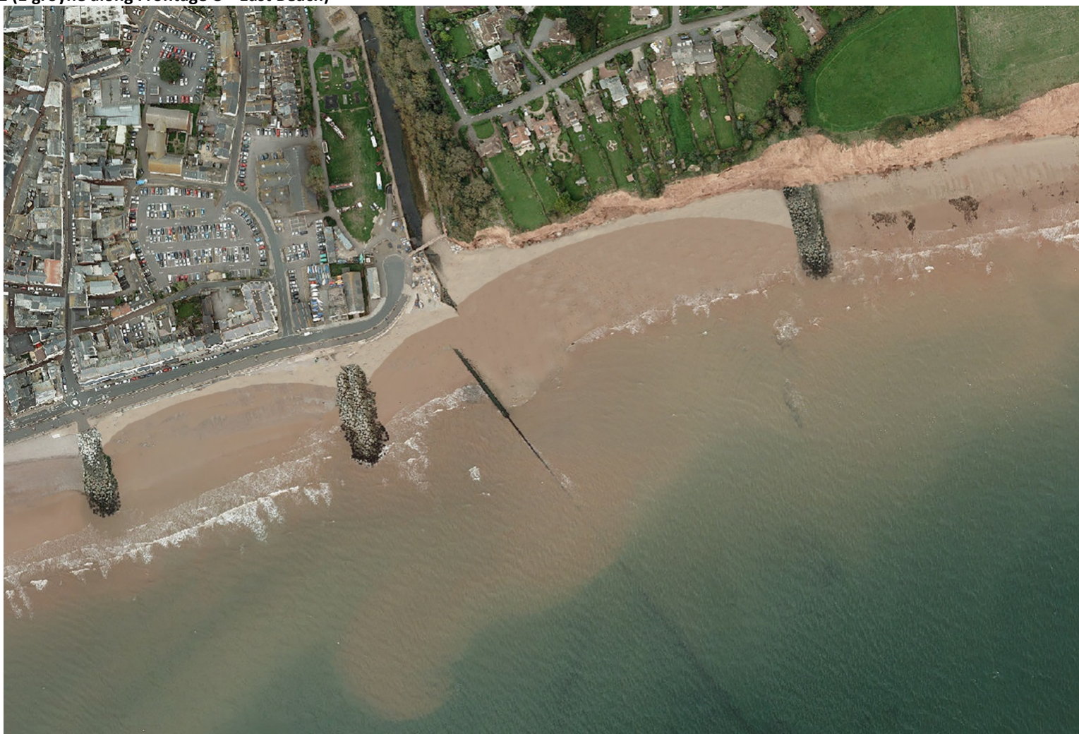
FIGURE G-1 Short-list Option S1 (1 groyne along Frontage C – East Beach)
